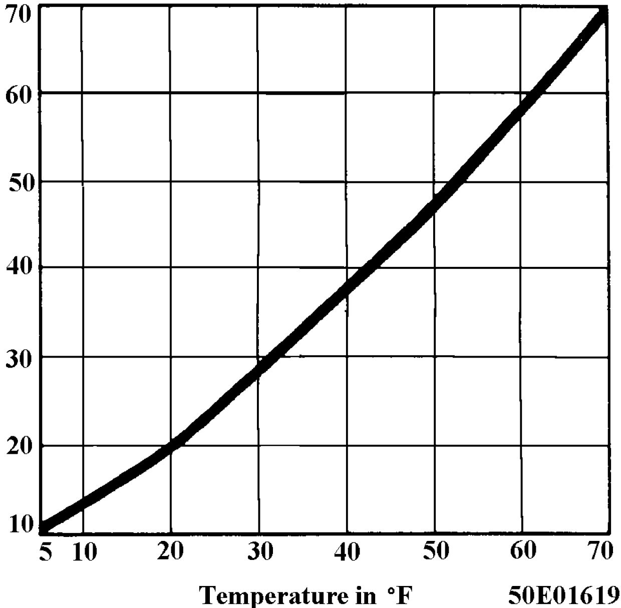
Fig. 2: Evaporator Temperature/Pressure A/C Chart
